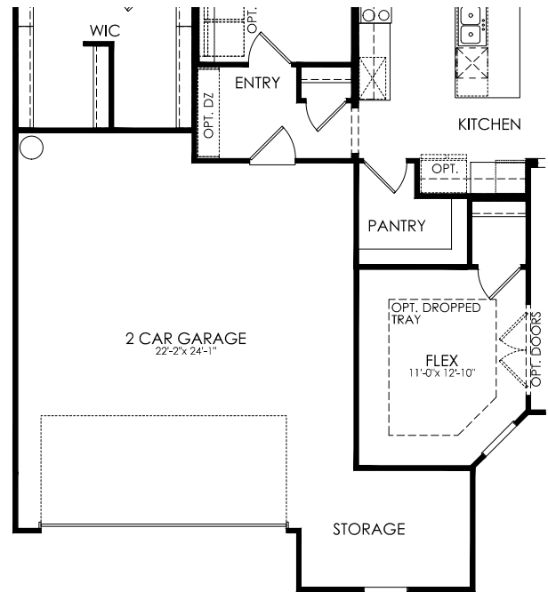
4' Garage Extension
